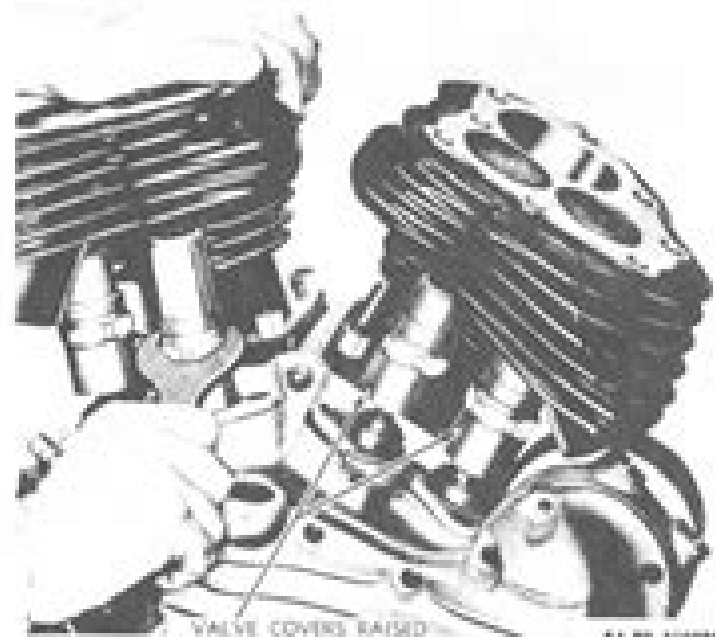
Figure 3—Freeing Valve Covers with Wrench (41-W-3637)
