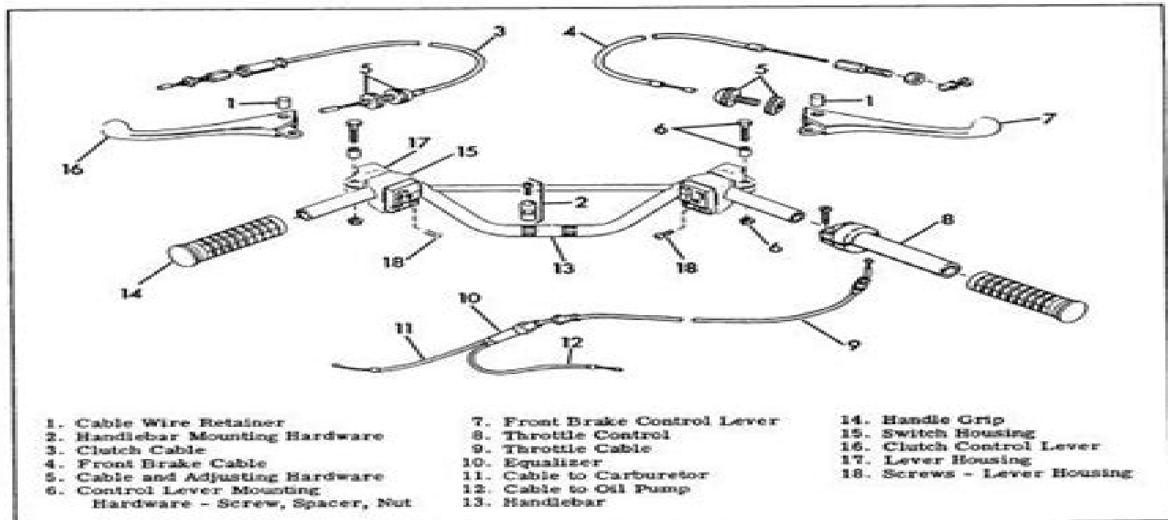
Figure 2.18. Handlebar and Associated Components
