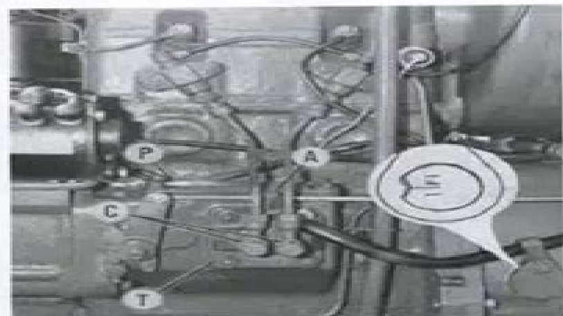
Fig. 50— Installed view of injection pump on Model L210. Inset shows flywheel timing mark for number 1 piston firing position.
