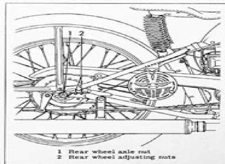
Figure 2B-8. Rear Chain Adjustment
