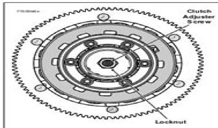
Figure 1-9. Clutch Assembly
