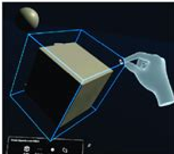
Object scaling
