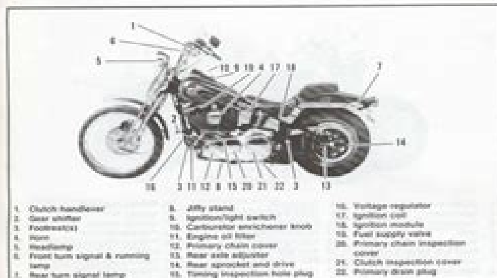
FIGURE 1-5. 1991 FXSTB - Left Side View
