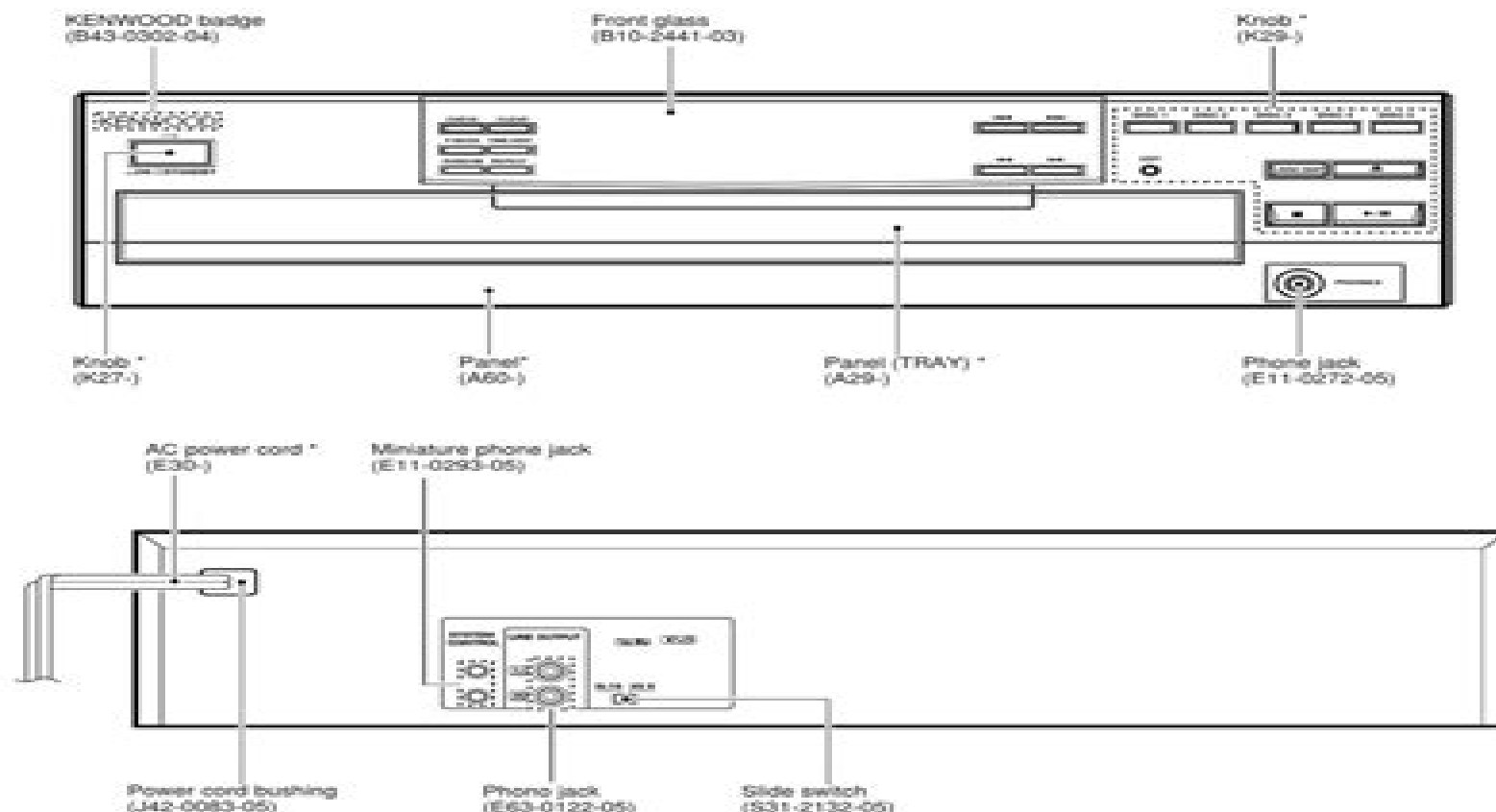
Illust is CD-204/DPF-R4010/DPF-R4010E. * Refer to parts list on page 16.
