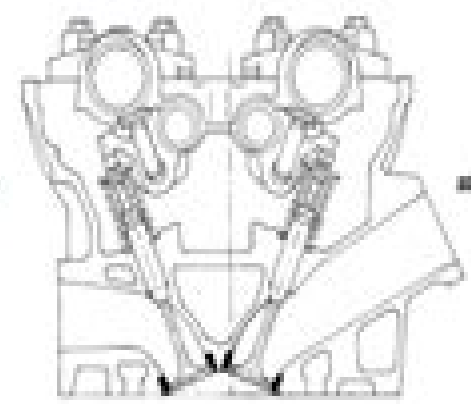
Cylinder head section
