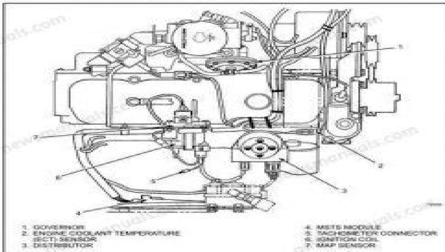
FIGURE 1. MSTS ARRANGEMENT IN THE ENGINE COMPARTMENT
