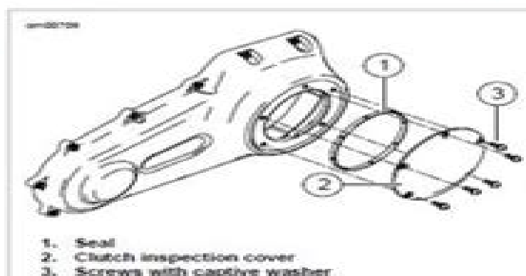
Figure 1-11. Clutch Cover
