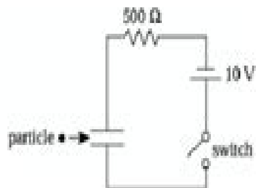
Figure 1 Circuit
