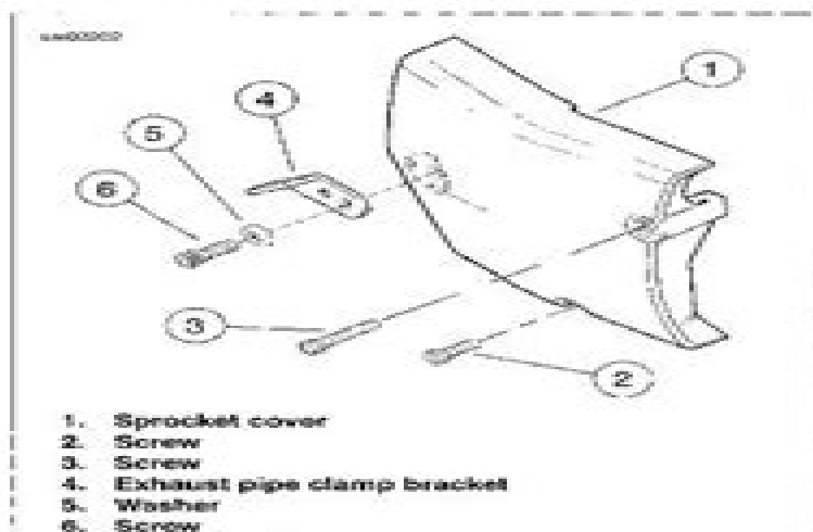
Figure 4-71. Sprocket Cover
