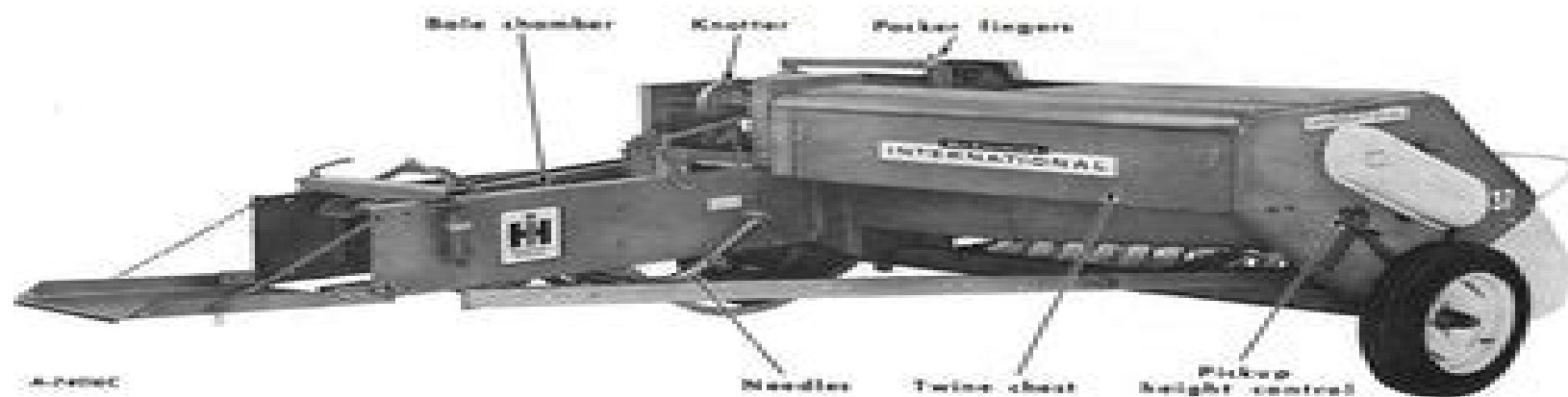
Illustr. 2A Right rear view of the 37 Twine Baler.
