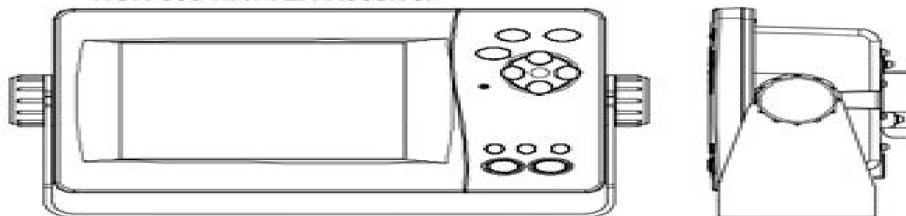
NCR-333 NAVTEX Receiver
