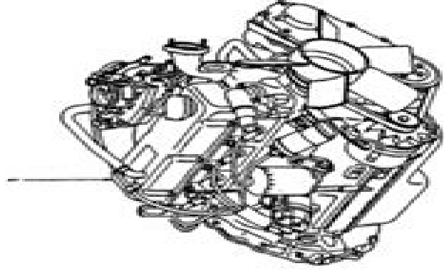
REAR LEFT SIDE VIEW
