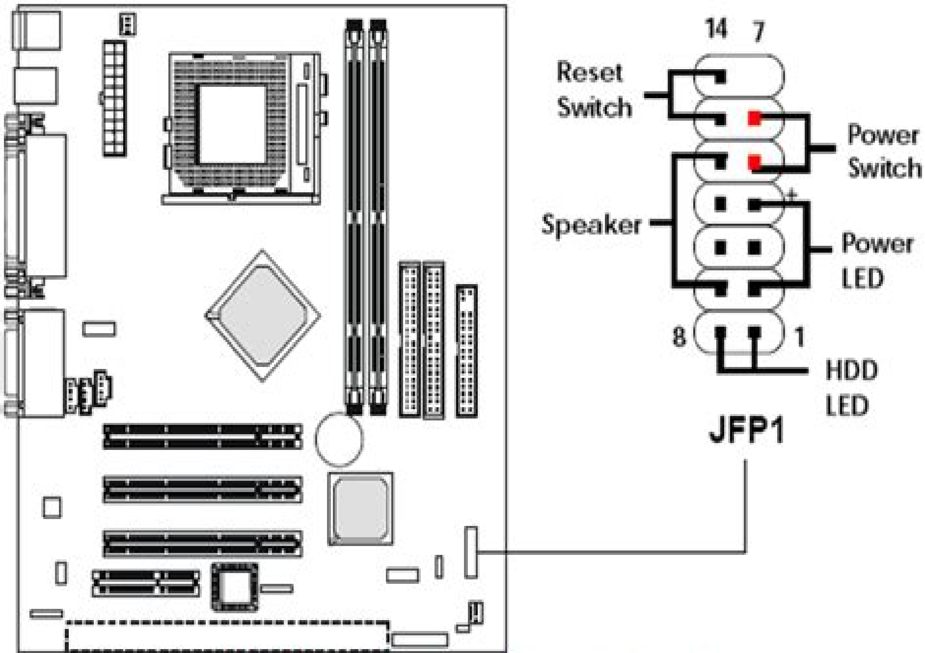
MSI MS-6368 front panel connection header
