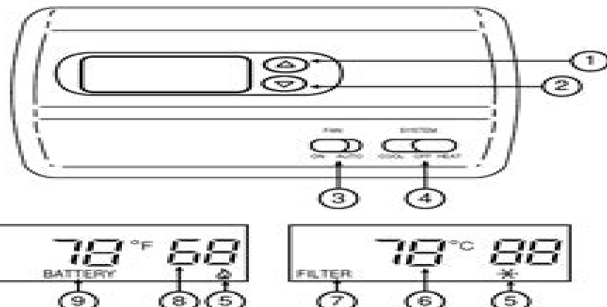
Figure 8. Thermostat display, buttons, and switches
