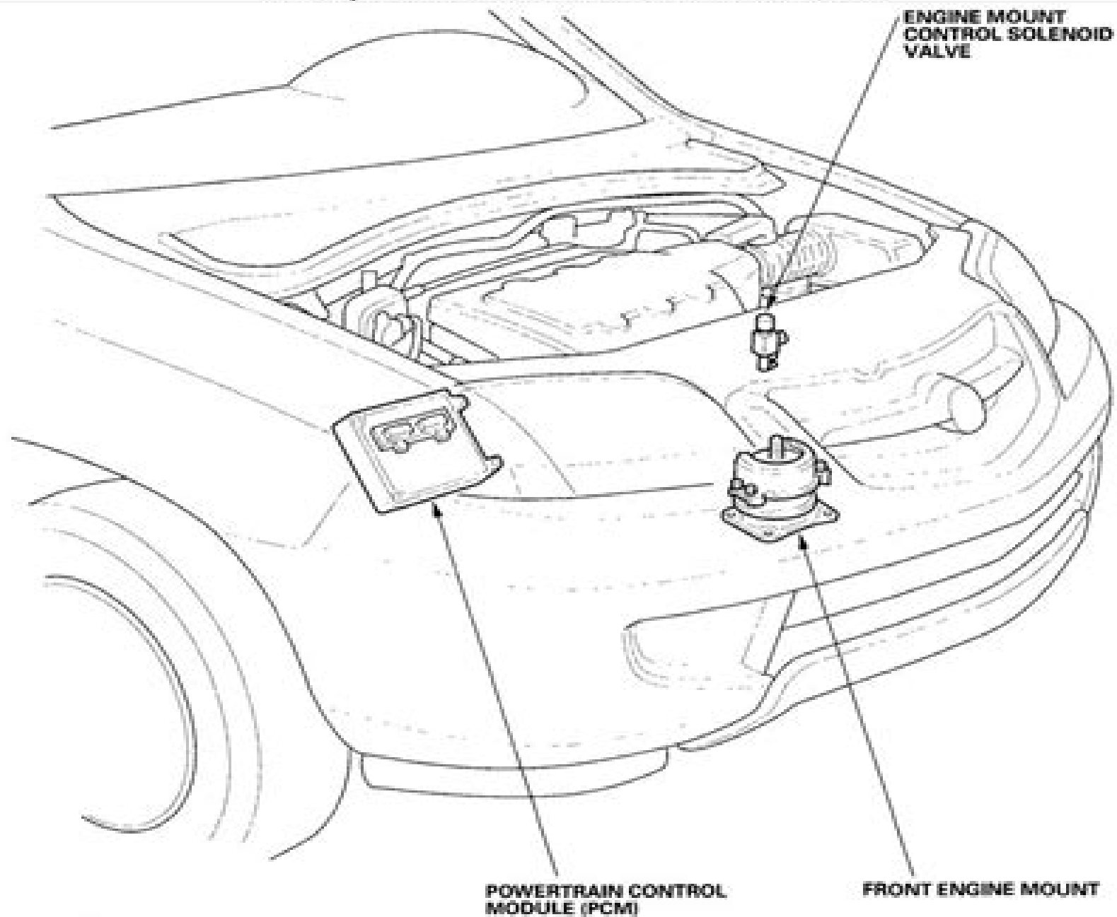
Fig. 1: Identifying Engine Mount Control System Components
