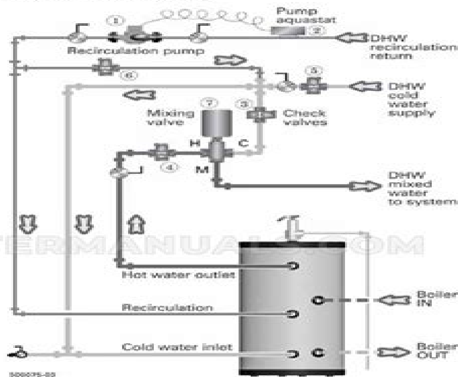
Figure 6 Recirculation piping
