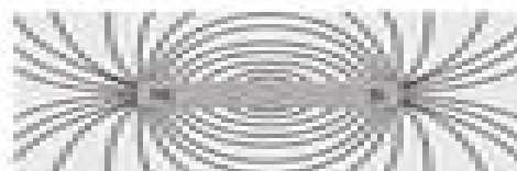
Magnetic field lines show the shape of the magnetic field around a magnet.
