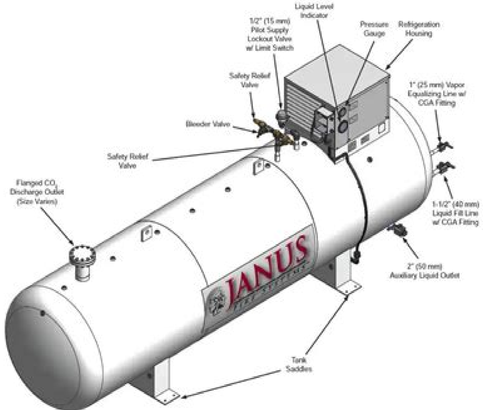
Typical Low Pressure Carbon Dioxide Storage Unit
