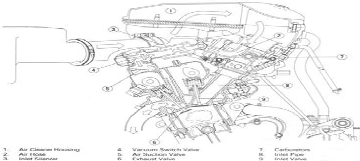
Secondary Air Injection System
