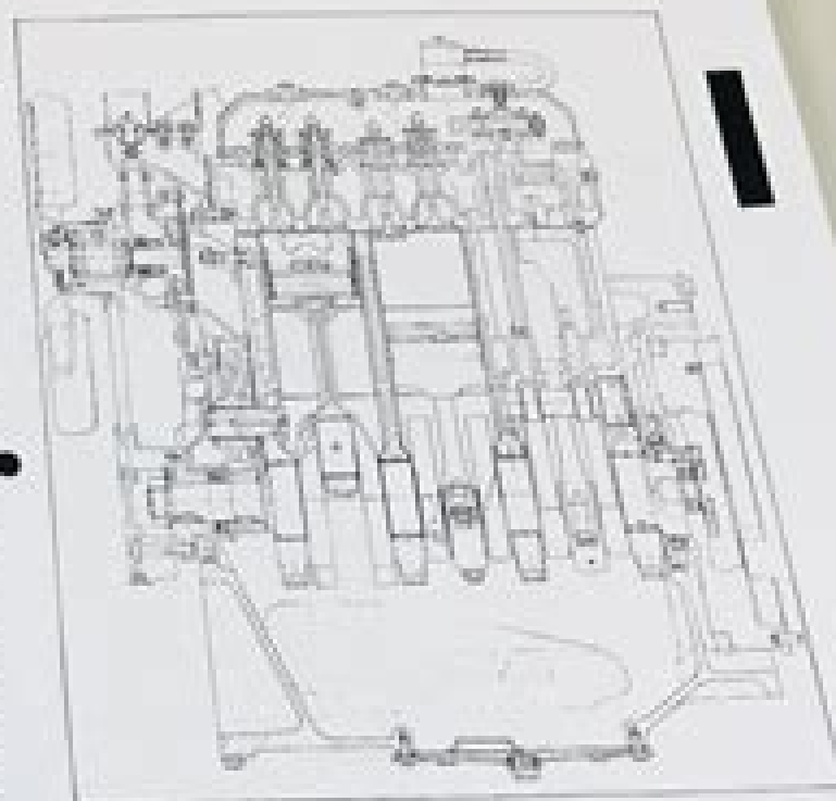
FIG. A-60A ENGINE - SECTIONAL VIEW
