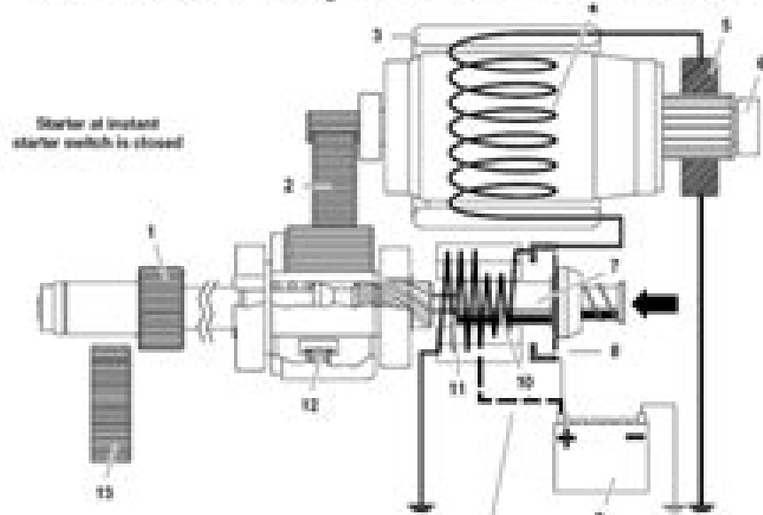
Starting circuit-see wiring diagram
