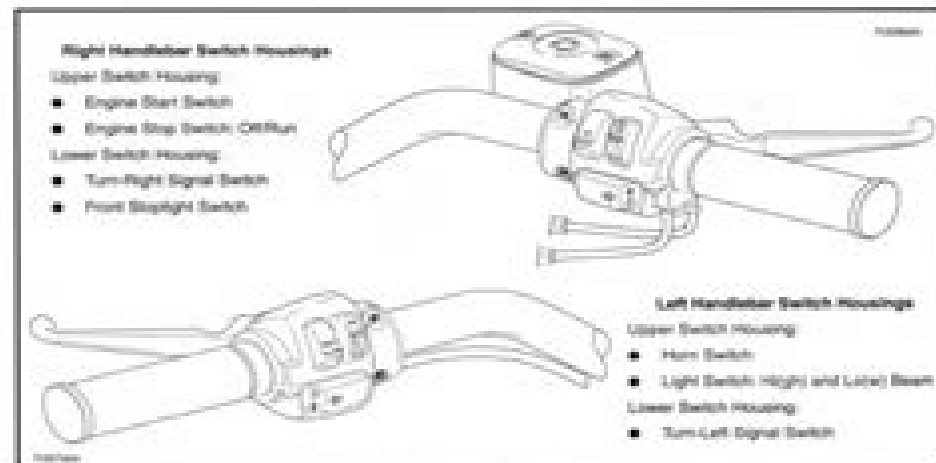
Figure 8-115. Road King Handlebar Switch Assemblies
