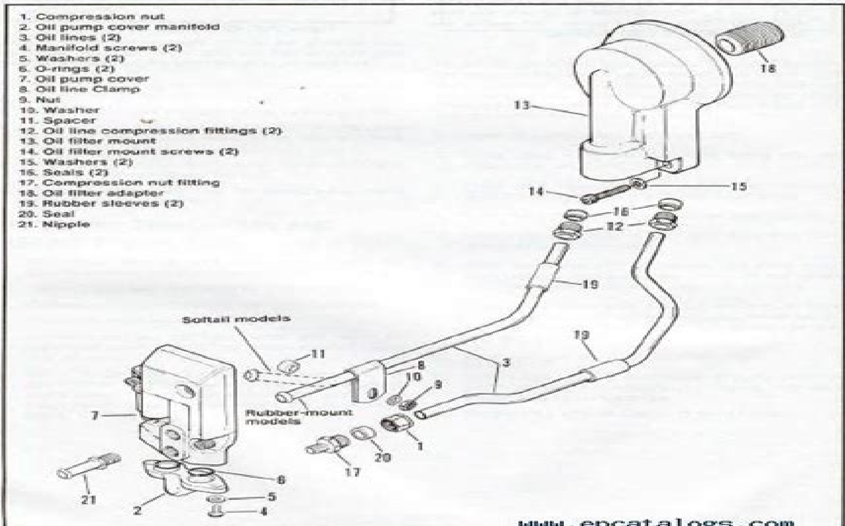
Figure 3-38. Oil Filter Mount and Oil Pump Cover - 1992
