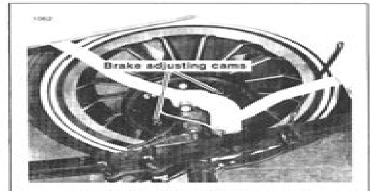
Figure 3-1. Brake Shoe Adjustment
