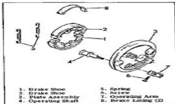
Figure 2.33. Disassembling Front Brake
