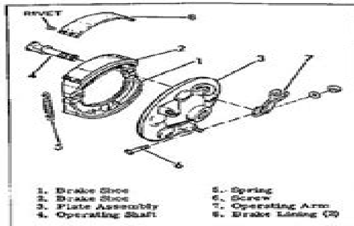
Figure 2.34. Disassembling Rear Brake
