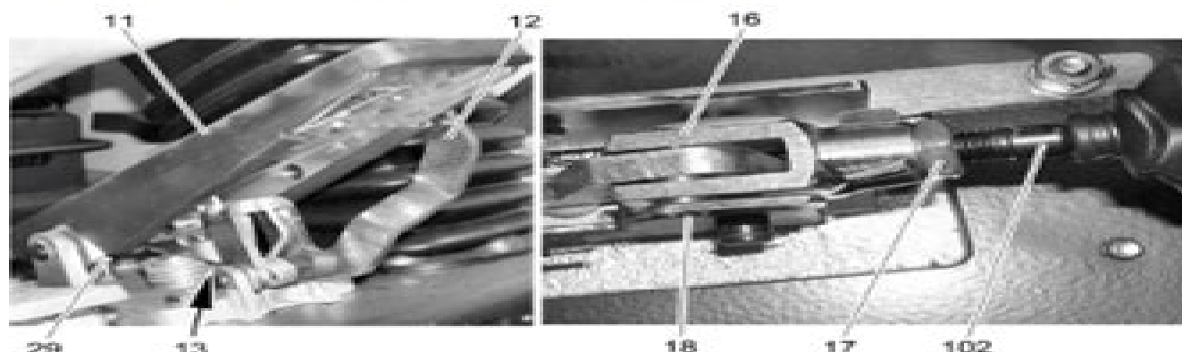
Fig. 43 Brake pedal and operating linkage of the brake valve at the compact brake block
