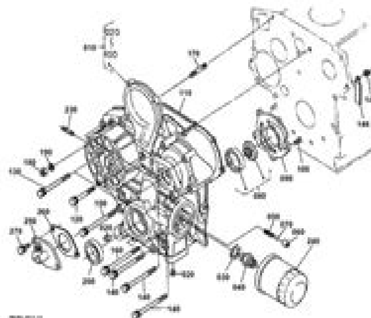
GEAR CASE
