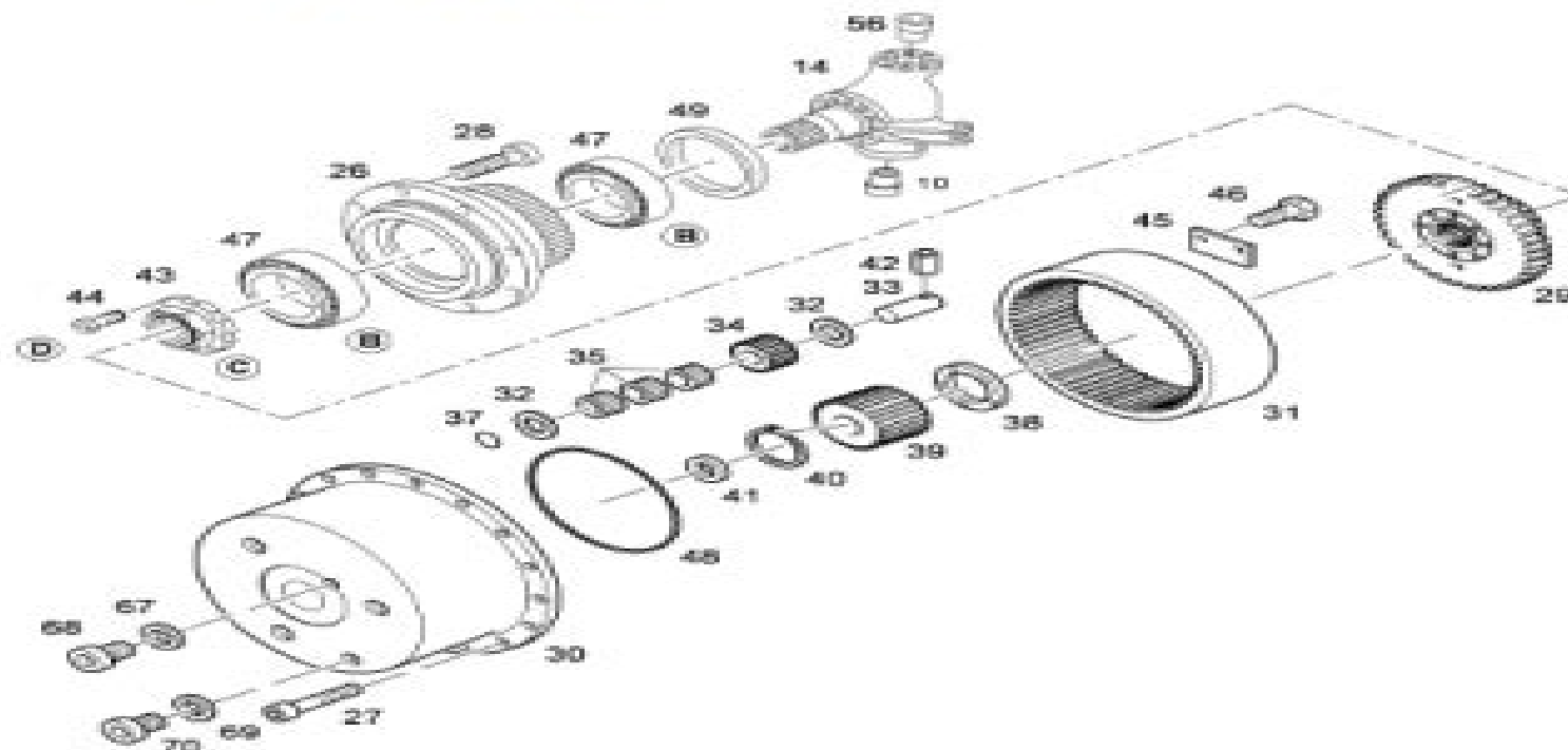
Fig. 6 Wheel bearing, planetary gear
