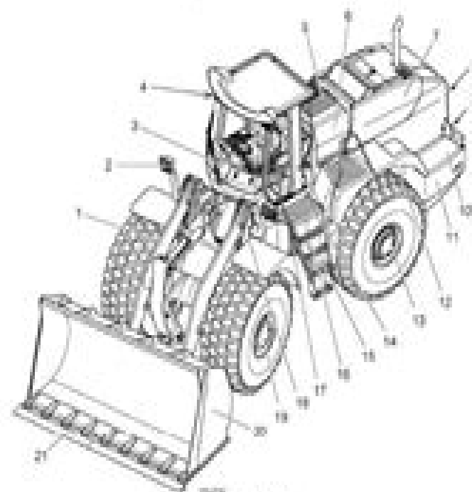
Figure 1 Left side of machine
