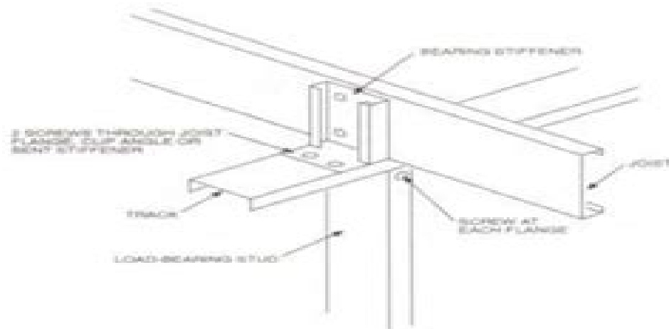
FIGURE R505.3.1(7) CONTINUOUS JOIST SPAN SUPPORTED ON STUD
