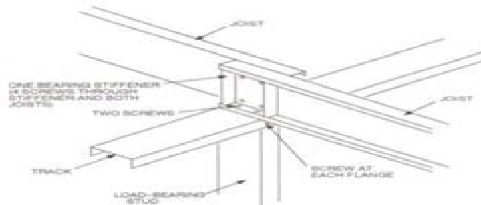
FIGURE R505.3.1(8) LAPPED JOISTS SUPPORTED ON STUD
