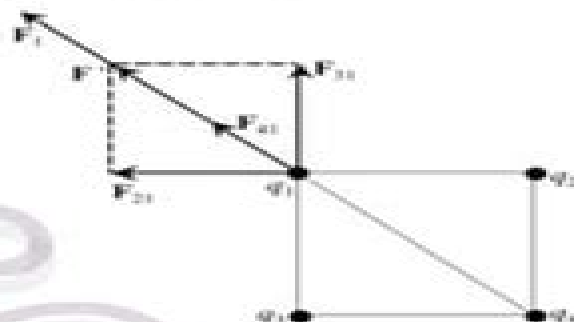
Figure 1S.1 Forces acting on charge q_1 from charges q_2 , q_3 , and q_4 .
