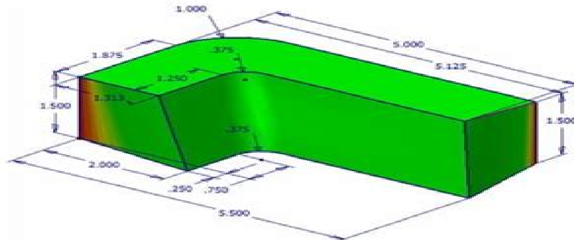
Figure 1: Mold Core Insert
