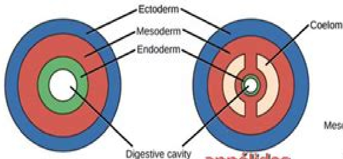
annélides (b) Eucoelomate (annelids, mollusks, arthropods, echinoderms, chordates)
