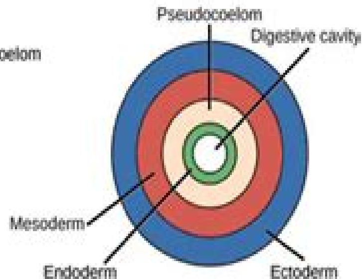
(c) Pseudocoelomate (roundworms)
