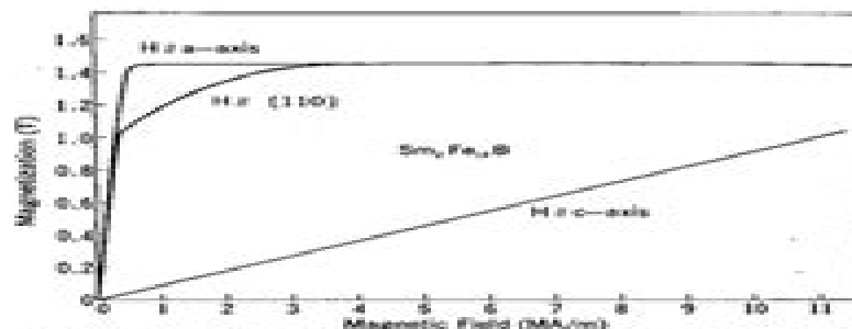
FIG. 2. Magnetization vs magnetic field curves of a single crystal of \text{Sm}_2\text{Fe}_{14}\text{B} at room temperature.
