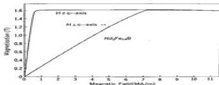
FIG. 1. Magnetization vs magnetic field curves of a single crystal of \text{Nd}_2\text{Fe}_{14}\text{B} at room temperature.
