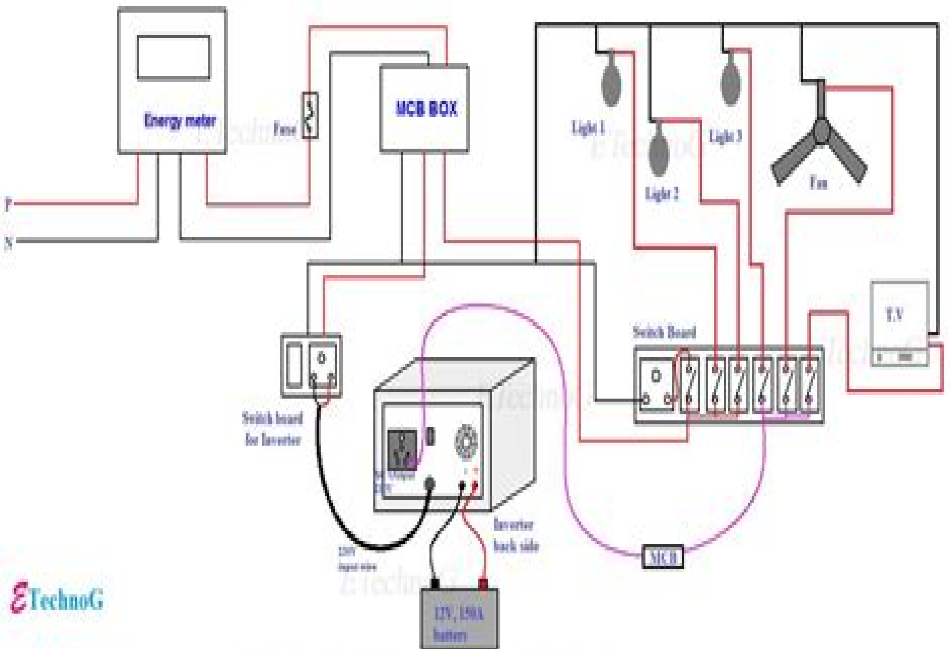
Inverter Wiring Diagram for Home
