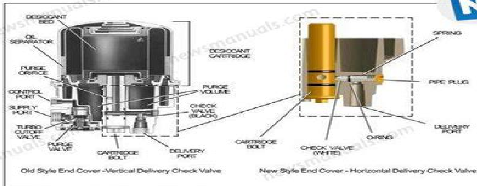
FIGURE 7 - AD-IP™ AIR DRYER SECTIONAL VIEW
