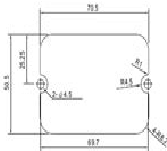
HOLE IN CHASSIS
