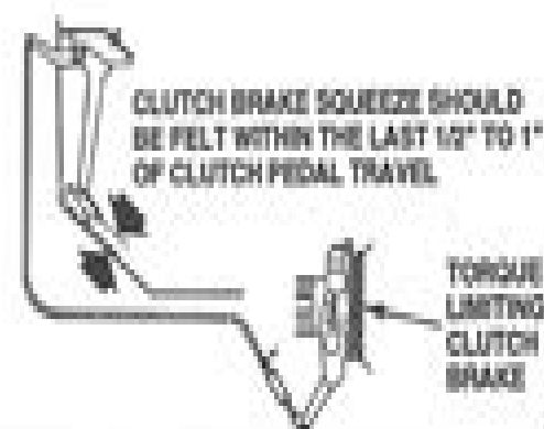
Figure 66 — Clutch Brake Squeeze (Spicer Easy Pedal)
