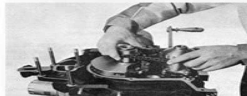
Fig. 1-79 Installing chain and sprockets
