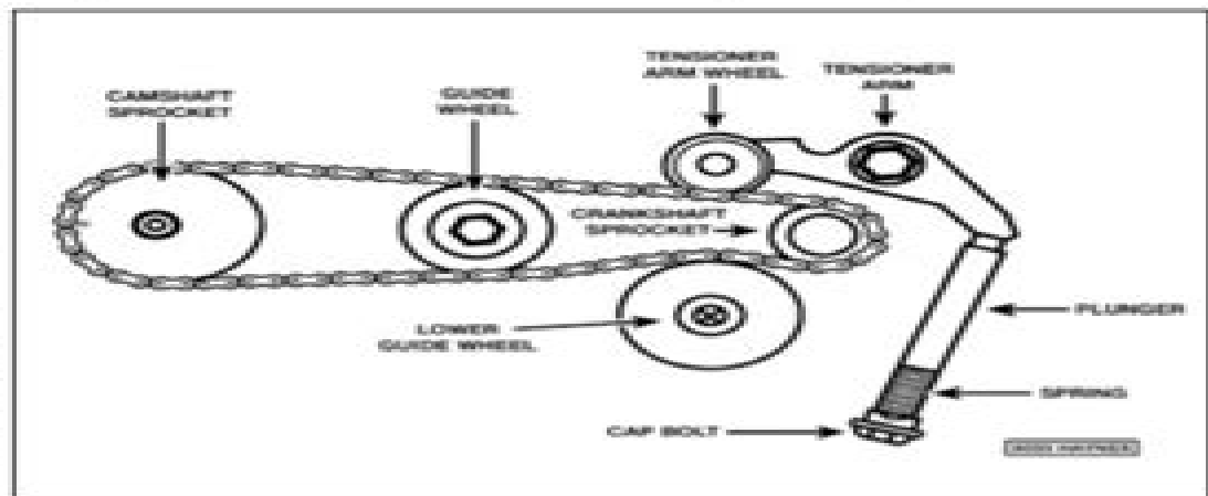
16.1 Cam chain tensioner components
