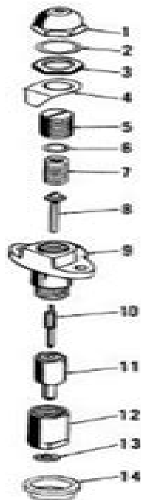
Fig. 154—Exploded view of C. A. V. injector nozzle and holder assembly. Correct opening pressure is indicated on tab (4).
