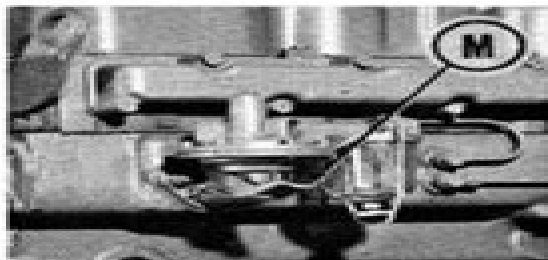
Fig. 150—Fuel lift pump showing manual lever (M).
