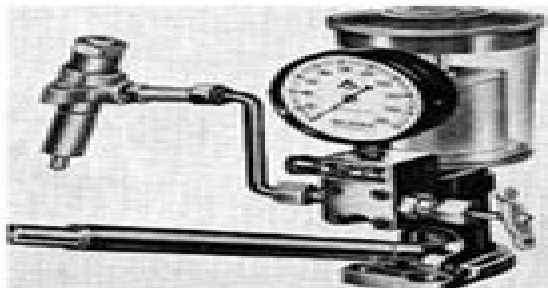
Fig. 151—A valveless injector tester is required to completely test and adjust the injector nozzles.
