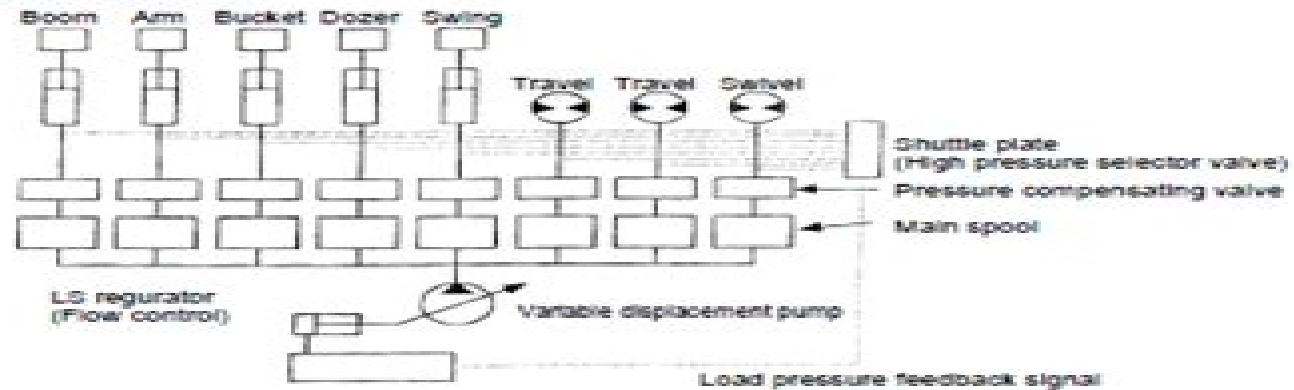
Hydraulic circuit outline
