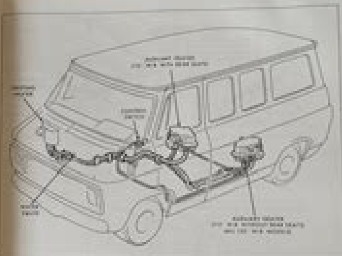
Fig. 10-Auxiliary Heater Installation
