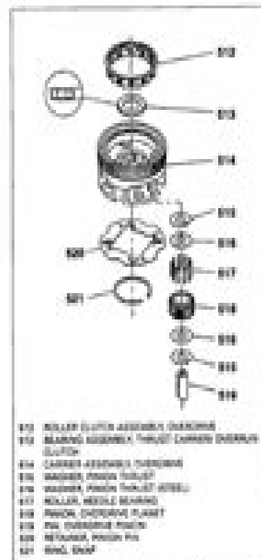
Figure 74. Overdrive Carrier Assembly
