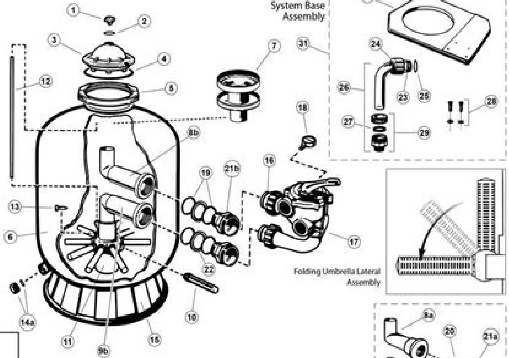
Original Side Mount Bulkhead Assembly (1995 and Prior)
