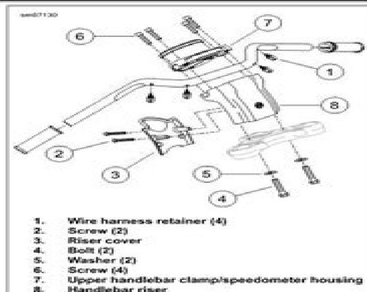
Figure 2-153. Handlebar: XL1200C
