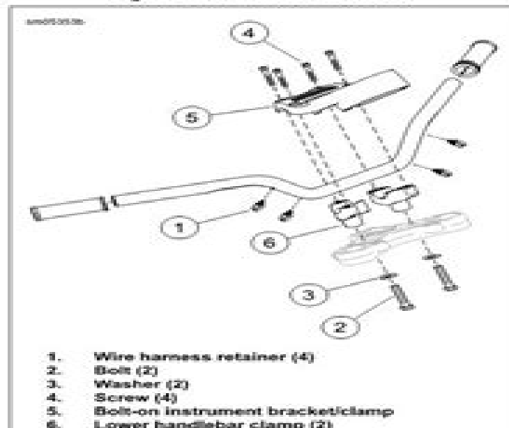
Figure 2-154. Handlebar: XL883N, XL1200CB, XL1200T
